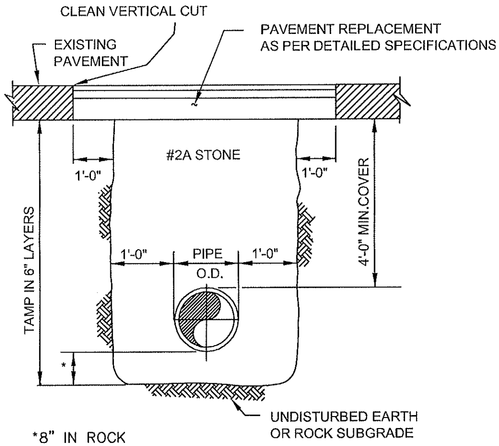
TYPICAL TRENCH FOR /BORO/ TOWNSHIP ROAD CROSSINGS AND & PAVED DRIVEWAYS
