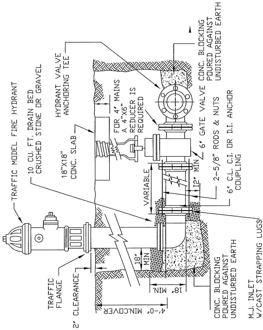
TYPICAL HYDRANT DETAIL
